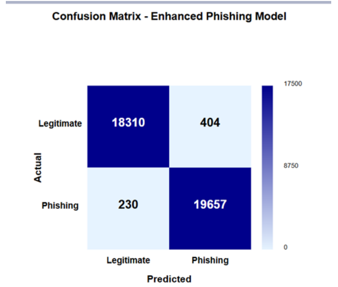
Fig. 5. Confusion matrix for the enhanced phishing detection model showing the distribution of predictions.
