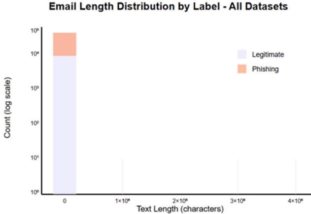
Fig. 7. Email length distribution by label (note logarithmic scale) showing concentration of both classes in shorter lengths.
