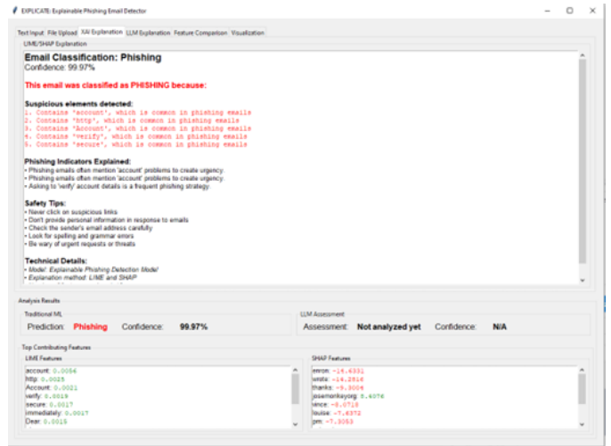
Fig. 9. EXPLICATE's standalone application interface showing the multi-tab analysis environment.
